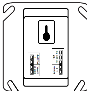
TX-6-ND rear view with Modular Connectors
